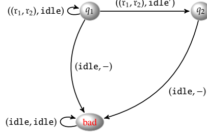
Figure 3: Partial description of \mathfrak{M}
